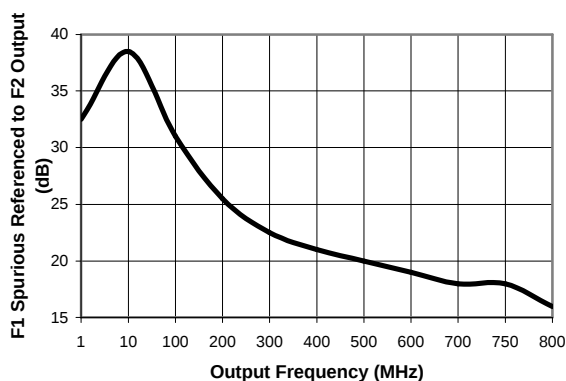
Spurious Response
